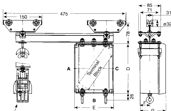
/ST-ST 2 R saddle for round cable
