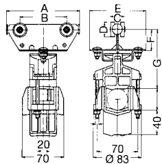
Bumper type
